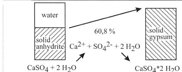
Figure 1. Chemical and physical basics of the anhydrite-gypsum conversion (M = molar mass, ρ = density, V = volume) (modified after Amstad & Kovari 2001).
