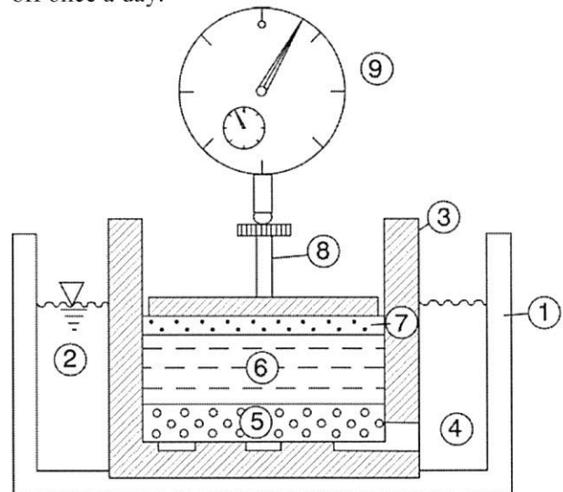
Figure 5. Drawing showing the test setup ("oedometercell") for the PST. 1 = water tray, 2 = water, 3 = swelling cell, 4 = drainage hole, 5 = lower porous plate, 6 = sample, 7 = upper porous plate, 8 = cap, 9 = dial gauge (after Thuro 1993).
